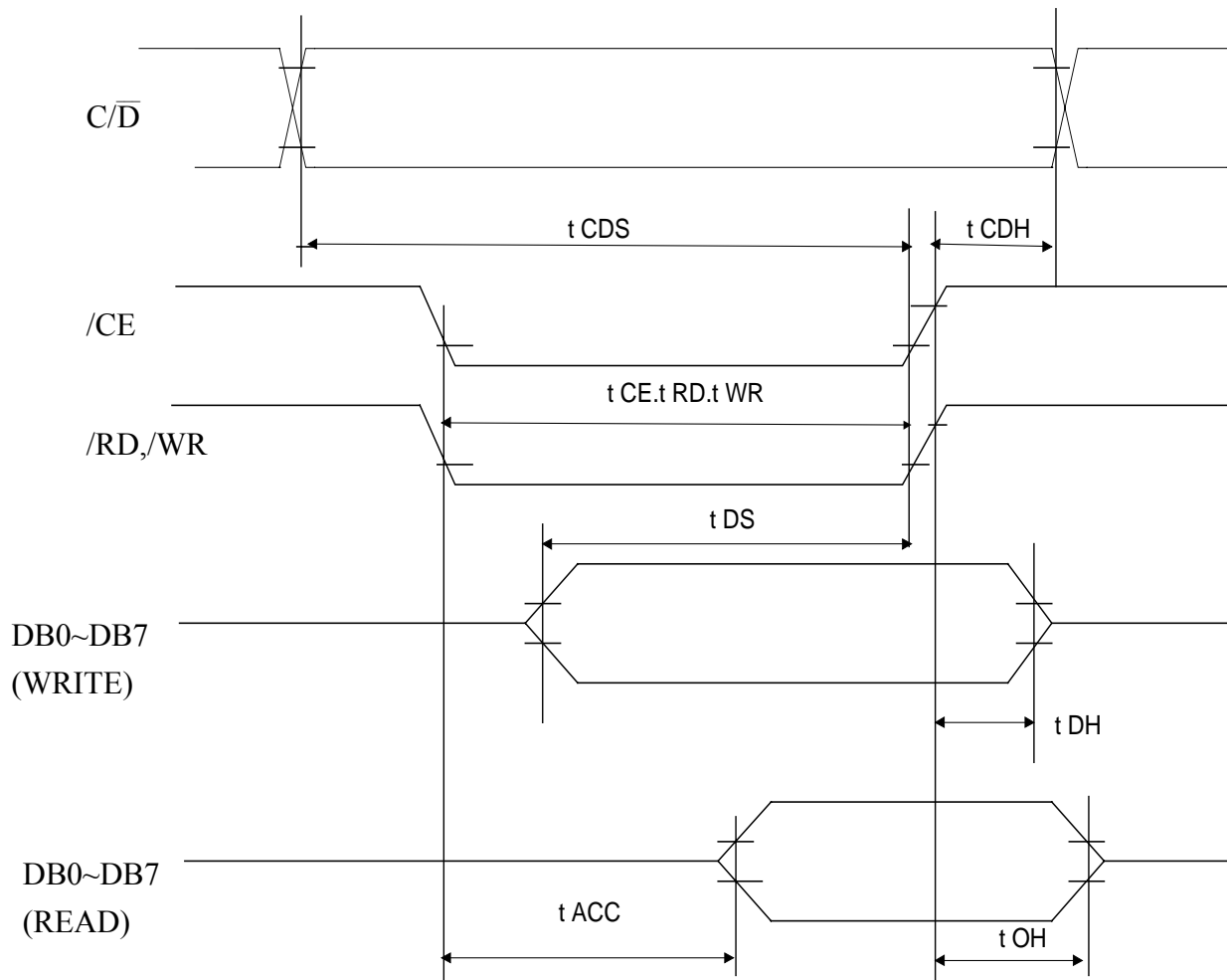
Figure 2: Bus Timing Diagram
